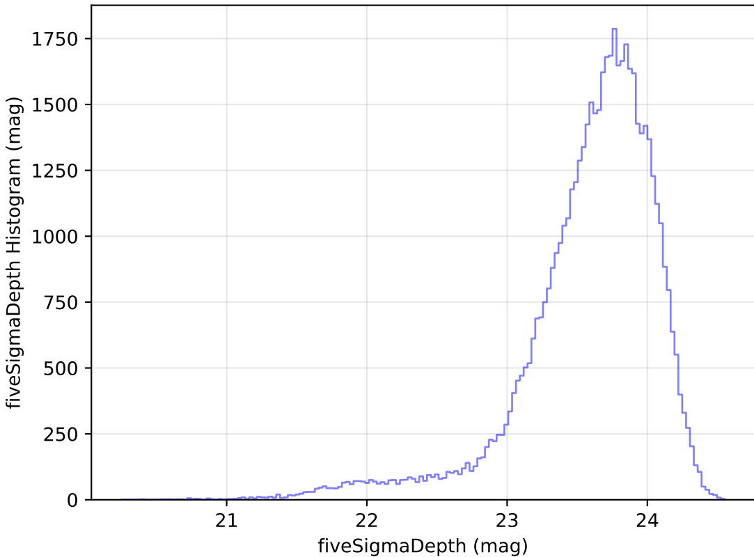
too_10_1v3.4_10yrs Yr 1 i band: fiveSigmaDepth Histogram
