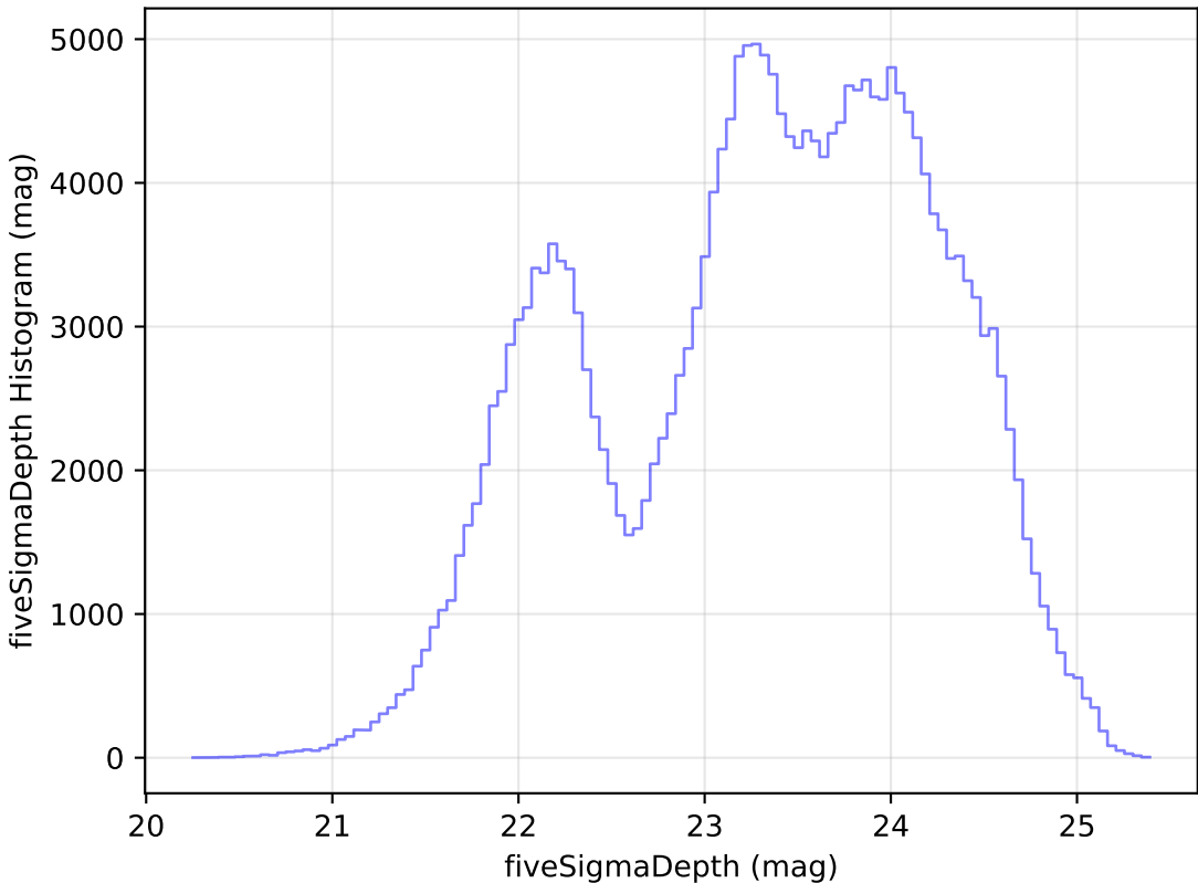
too_10_1v3.4_10yrs Yr 1 all bands: fiveSigmaDepth Histogram
