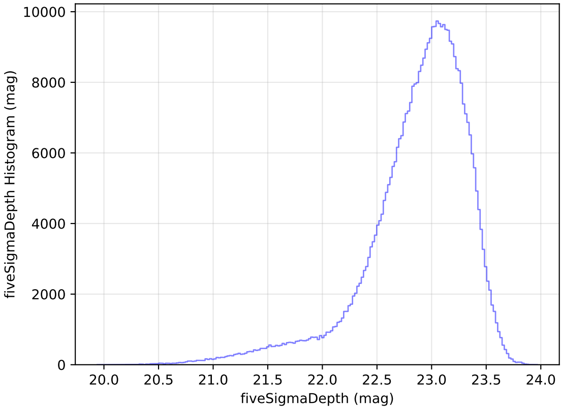
too_10_1v3.4_10yrs WFD z band: fiveSigmaDepth Histogram
