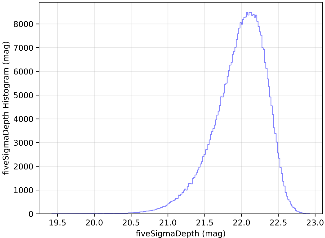
too_10_1v3.4_10yrs WFD y band: fiveSigmaDepth Histogram
