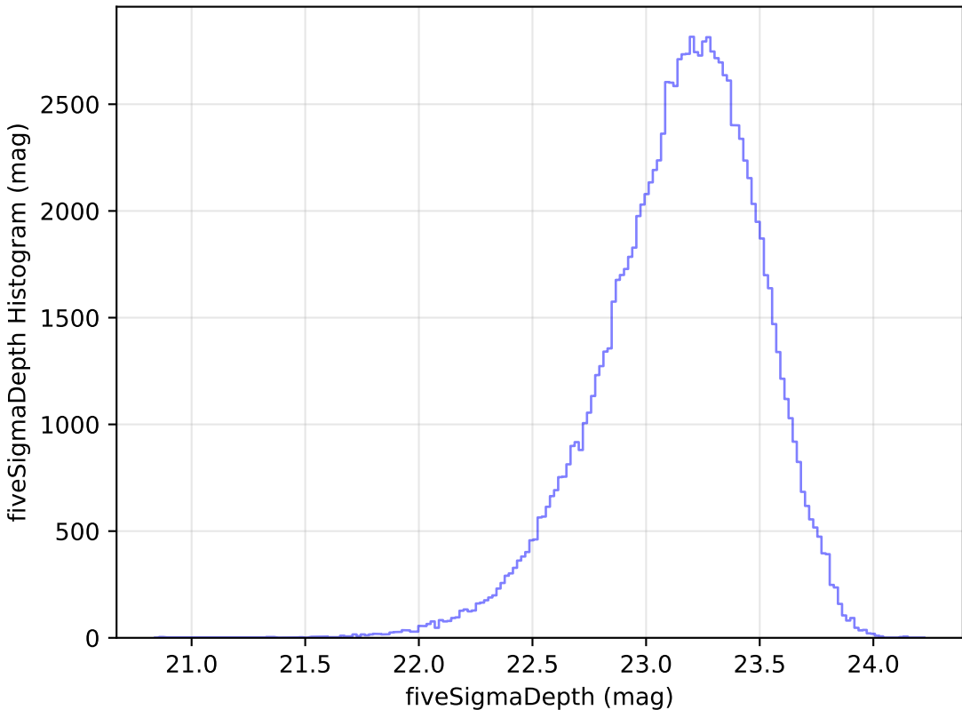
too_10_1v3.4_10yrs WFD u band: fiveSigmaDepth Histogram
