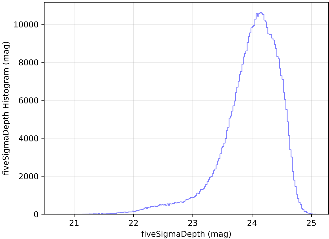
too_10_1v3.4_10yrs WFD r band: fiveSigmaDepth Histogram
