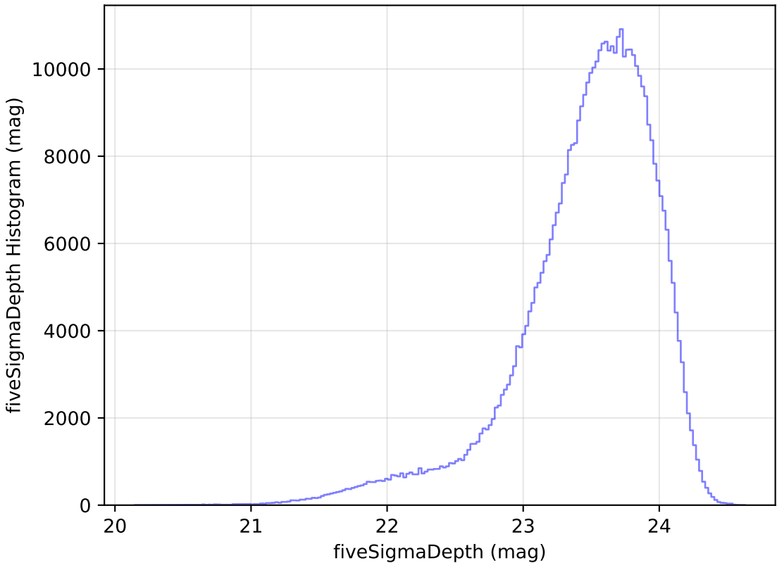
too_10_1v3.4_10yrs WFD i band: fiveSigmaDepth Histogram
