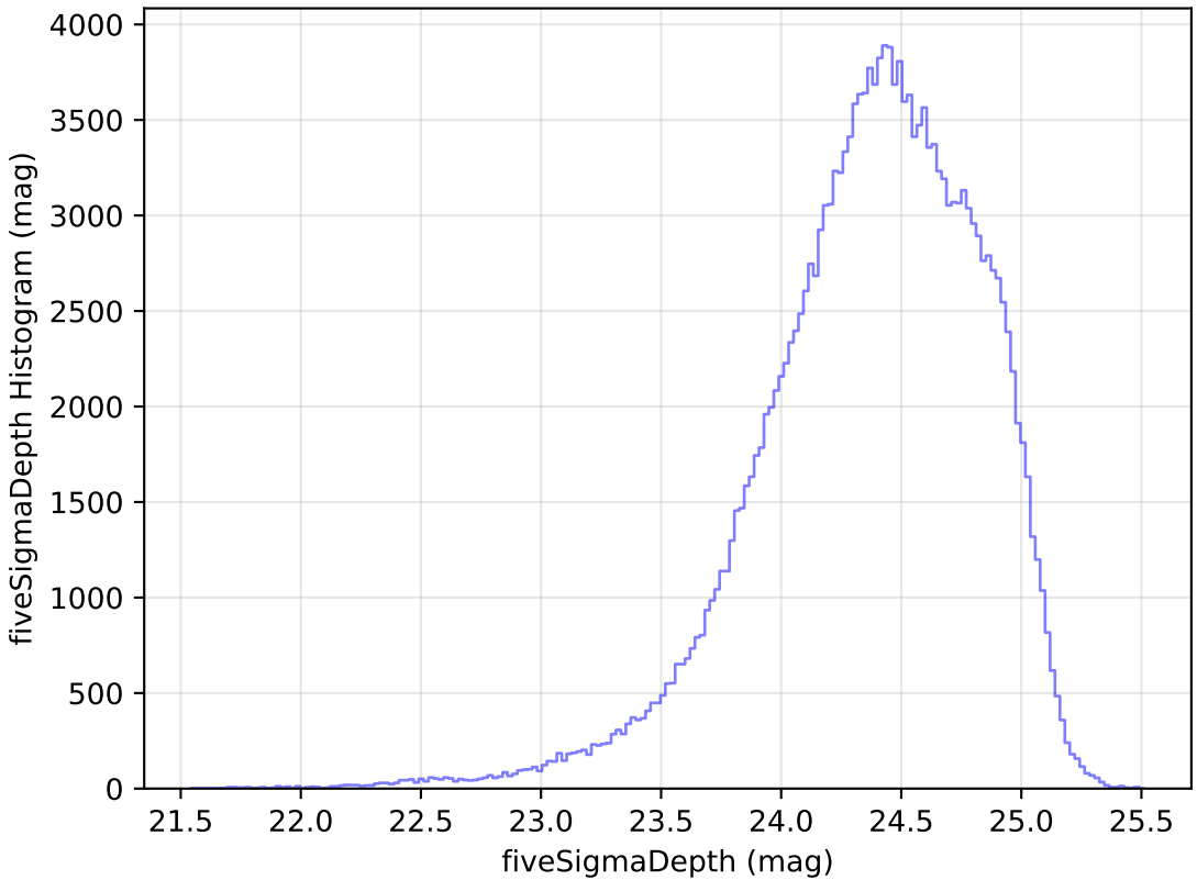
too_10_1v3.4_10yrs WFD g band: fiveSigmaDepth Histogram
