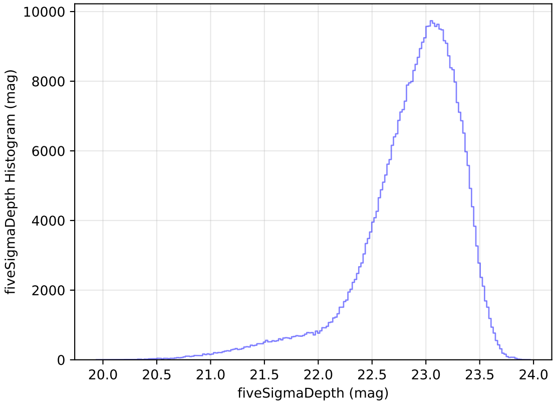
too_10_1v3.4_10yrs All sky z band: fiveSigmaDepth Histogram
