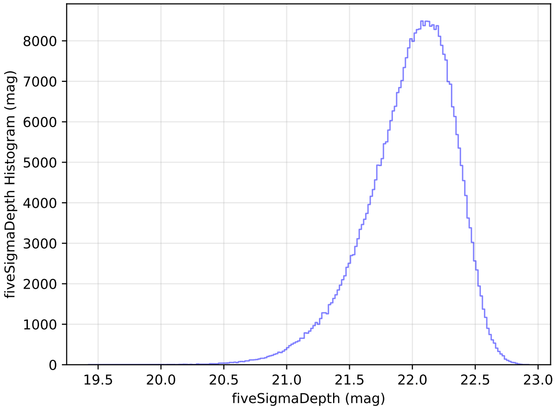
too_10_1v3.4_10yrs All sky y band: fiveSigmaDepth Histogram
