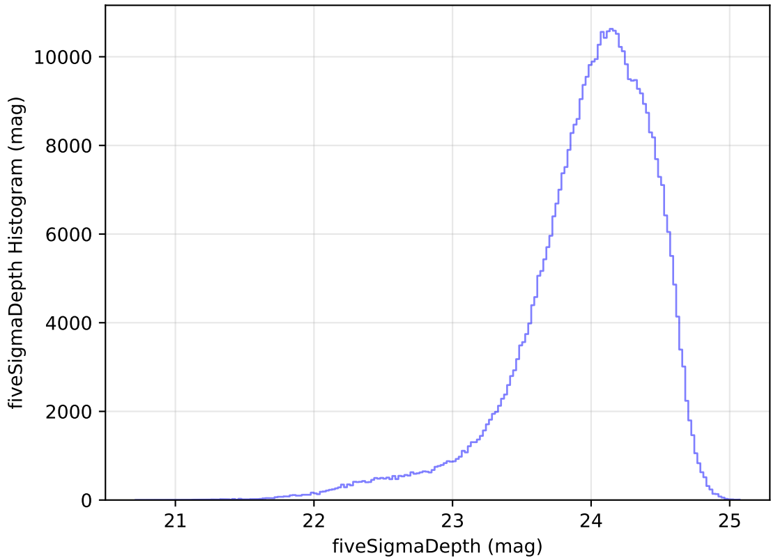
too_10_1v3.4_10yrs All sky r band: fiveSigmaDepth Histogram
