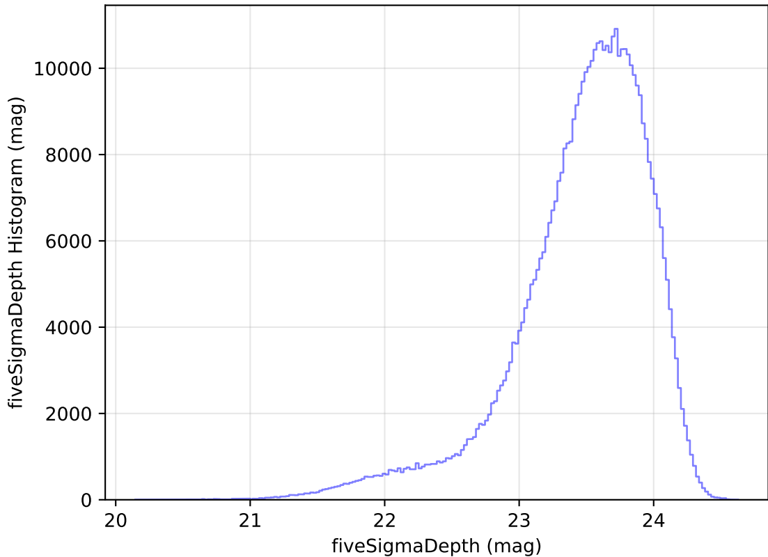
too_10_1v3.4_10yrs All sky i band: fiveSigmaDepth Histogram
