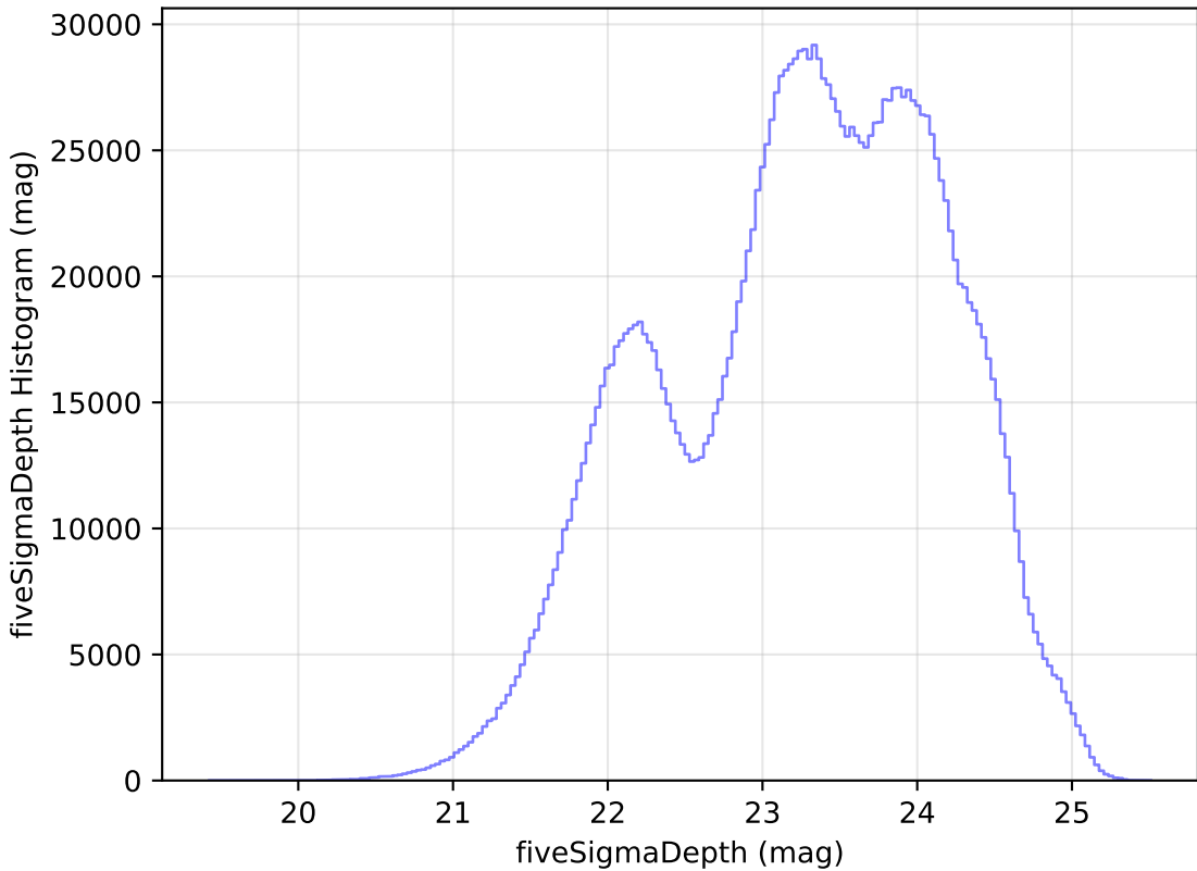
too_10_1v3.4_10yrs All sky all bands: fiveSigmaDepth Histogram
