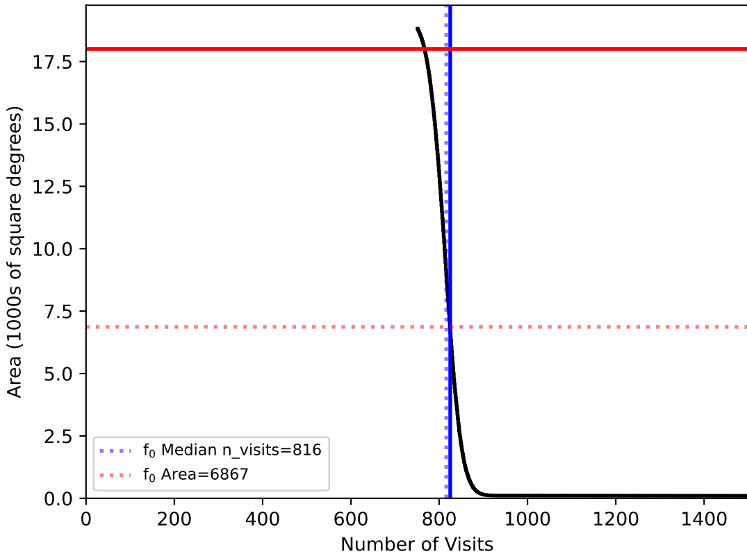
too_10_1v3.4_10yrs WFD: f0
