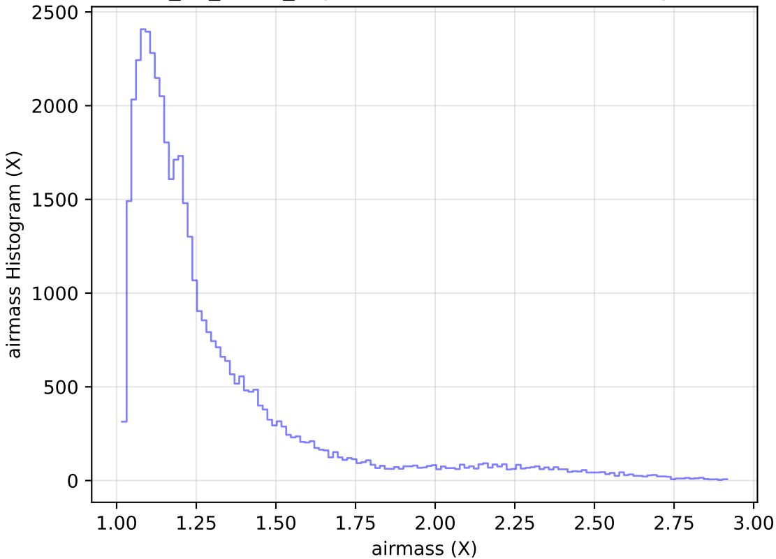
too_10_1v3.4_10yrs Yr 1 z band: airmass Histogram
