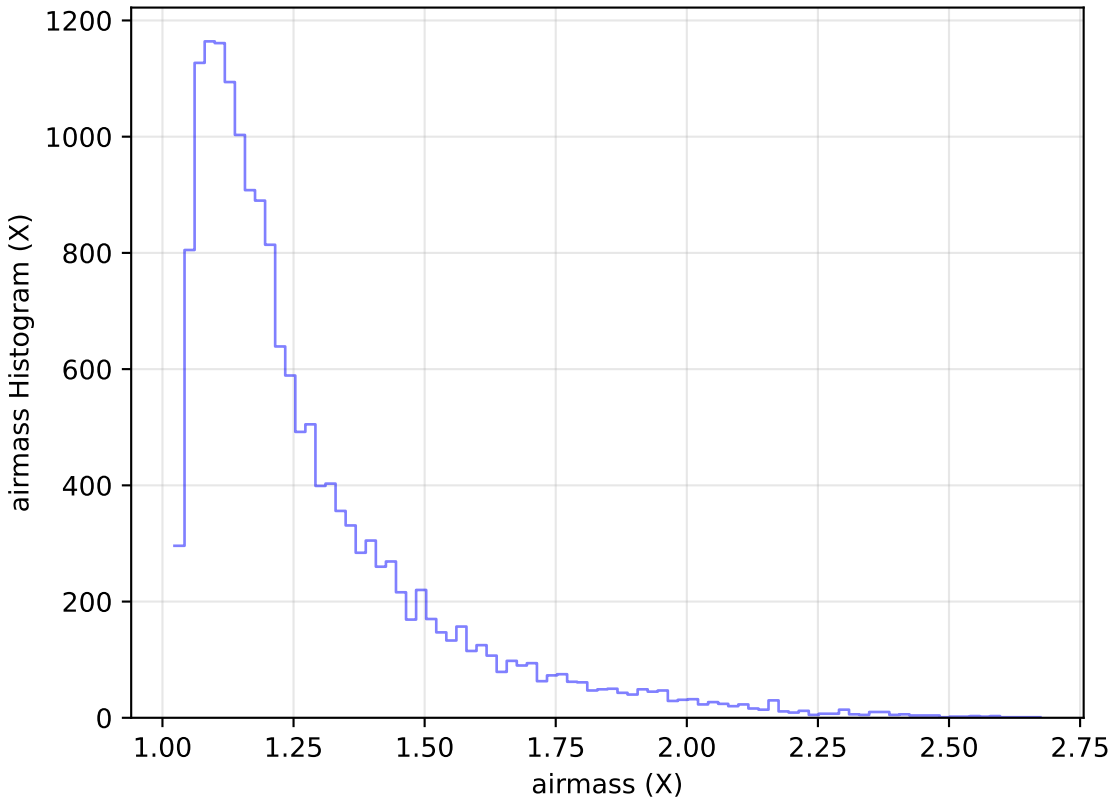
too_10_1v3.4_10yrs Yr 1 u band: airmass Histogram
