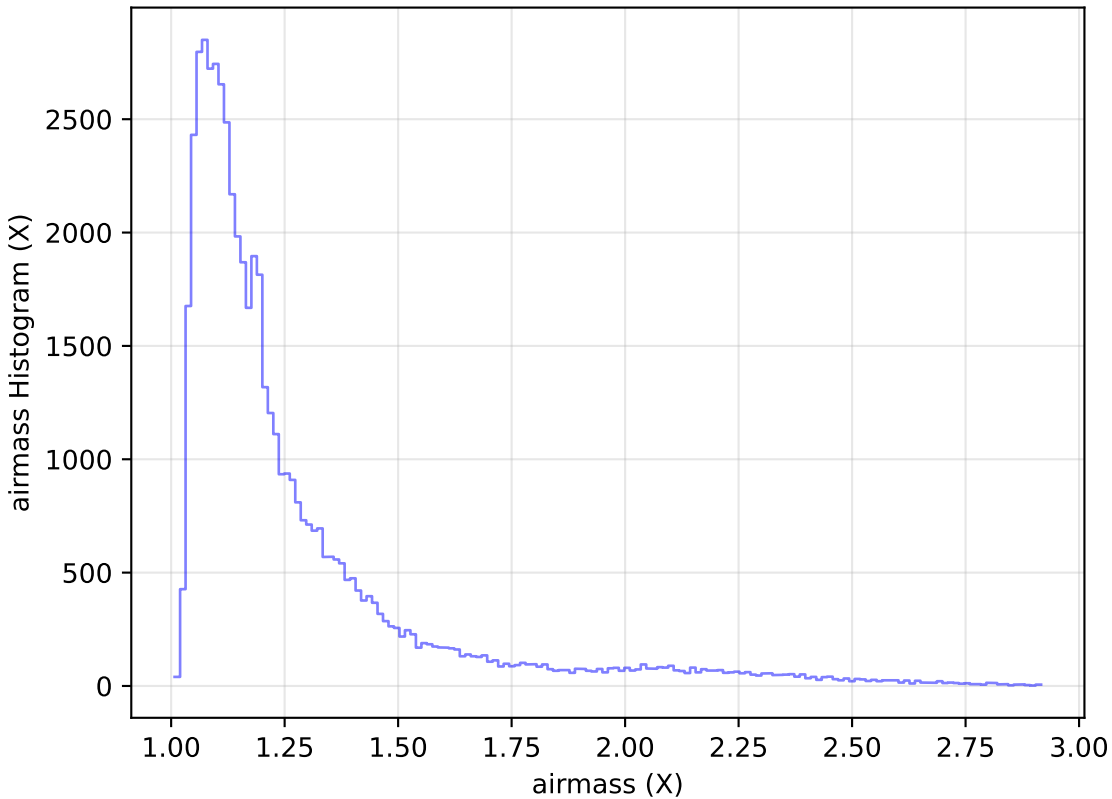
too_10_1v3.4_10yrs Yr 1 i band: airmass Histogram
