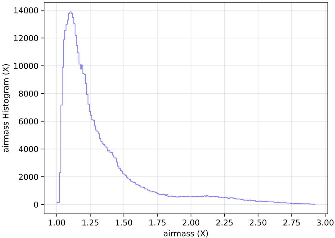
too_10_1v3.4_10yrs WFD z band: airmass Histogram
