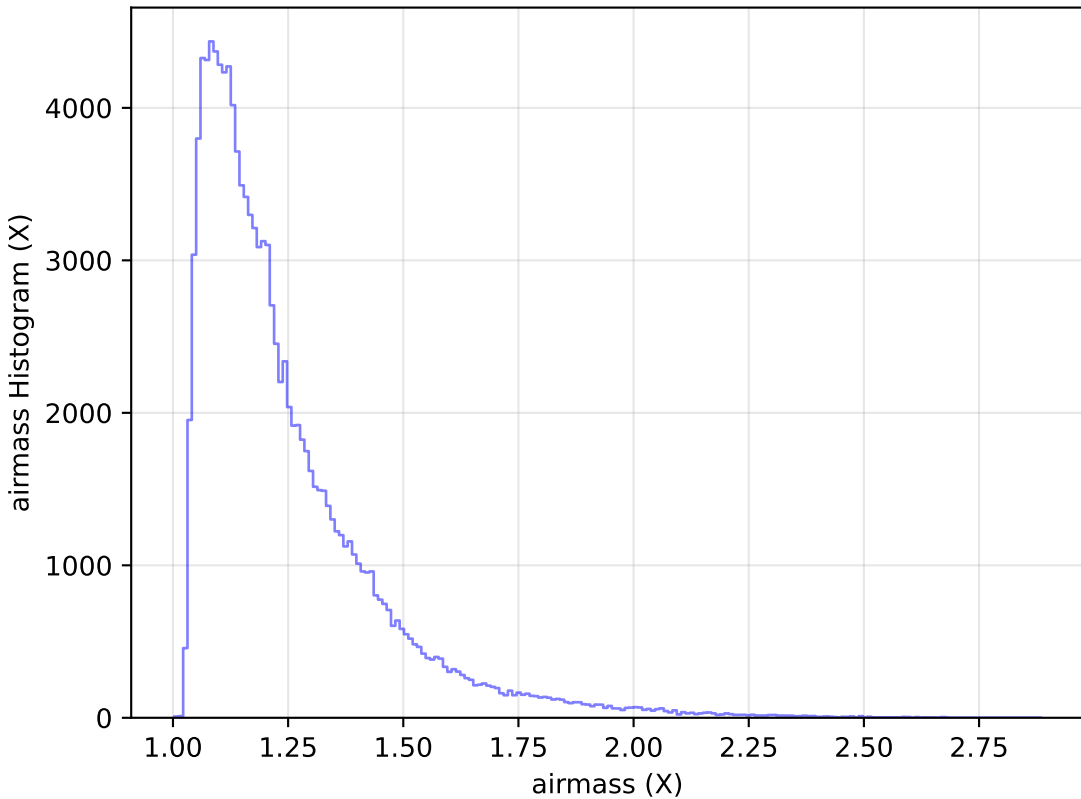
too_10_1v3.4_10yrs WFD u band: airmass Histogram
