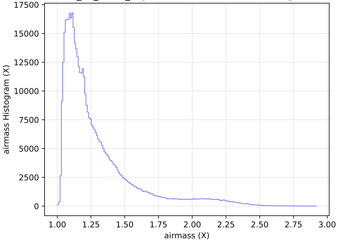
too_10_1v3.4_10yrs WFD r band: airmass Histogram
