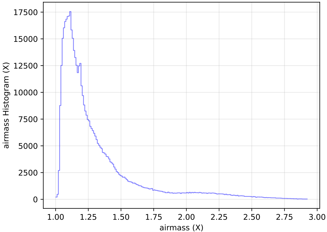
too_10_1v3.4_10yrs WFD i band: airmass Histogram
