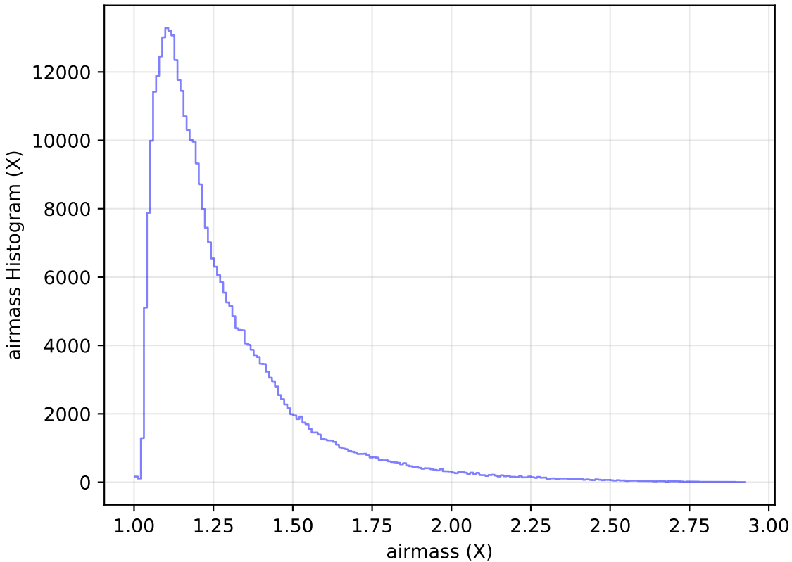
too_10_1v3.4_10yrs All sky y band: airmass Histogram
