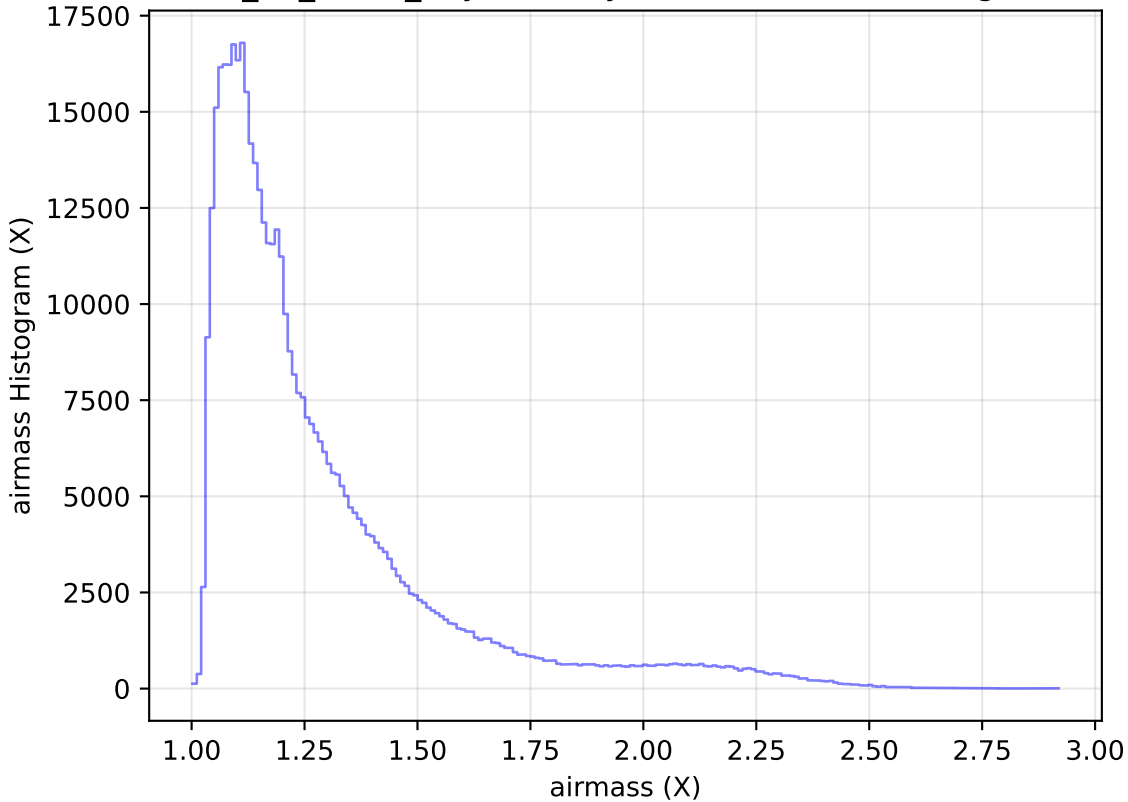
too_10_1v3.4_10yrs All sky r band: airmass Histogram
