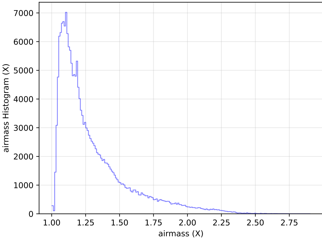
too_10_1v3.4_10yrs All sky g band: airmass Histogram
