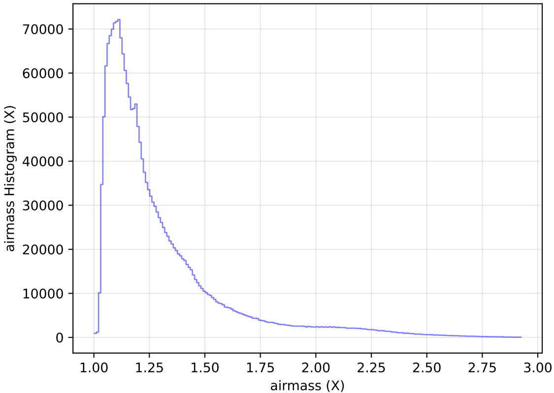
too_10_1v3.4_10yrs All sky all bands: airmass Histogram
