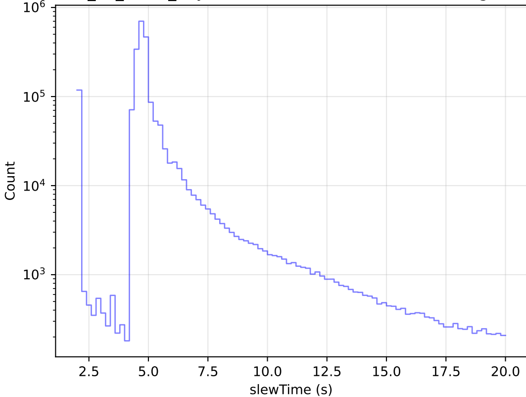
too_10_1v3.4_10yrs All visits: Zoom Slew Time Histogram
