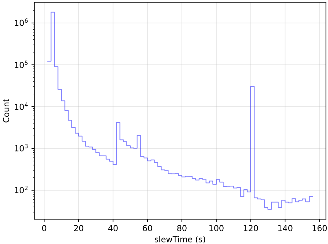
too_10_1v3.4_10yrs All visits: Slew Time Histogram
