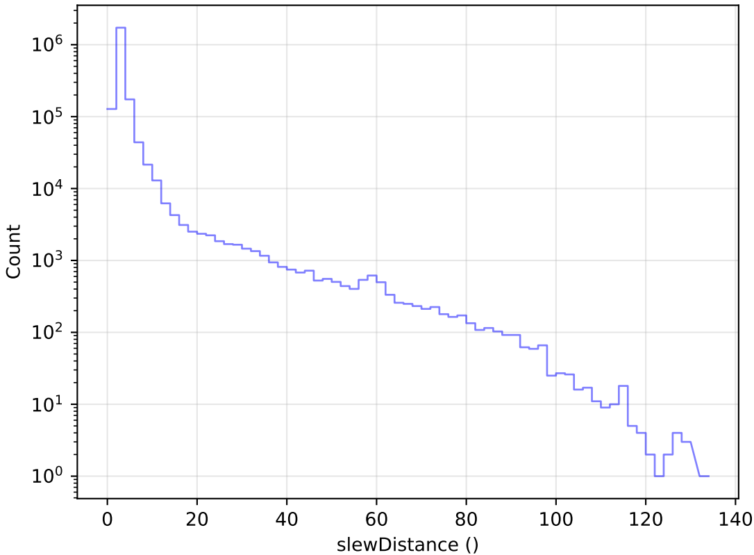
too_10_1v3.4_10yrs All visits: Slew Distance Histogram
