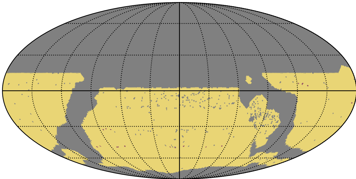
too_10_1v3.4_10yrs WFD: RapidRevisits
