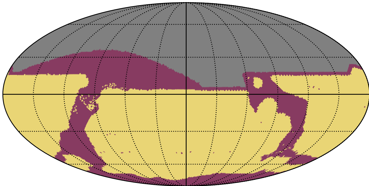
too_10_1v3.4_10yrs All sky: RapidRevisits
