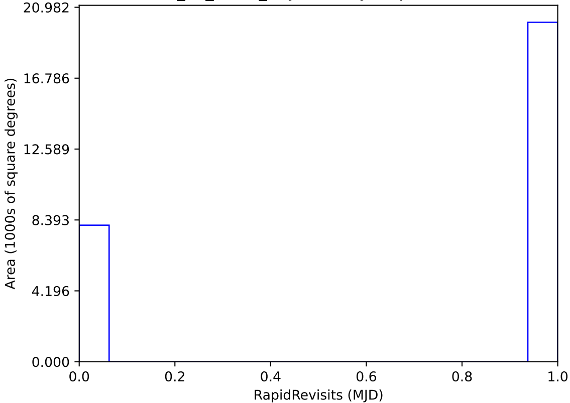
too_10_1v3.4_10yrs All sky: RapidRevisits
