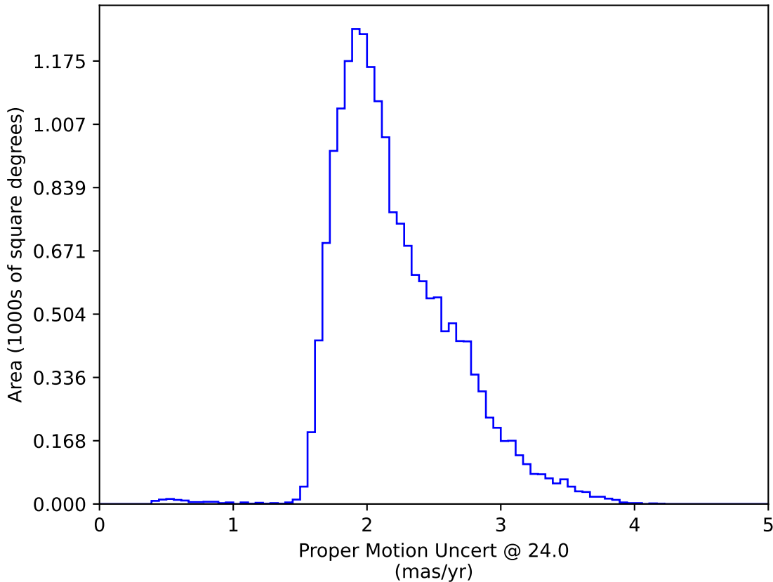
too_10_1v3.4_10yrs WFD: Proper Motion Uncert @ 24.0
