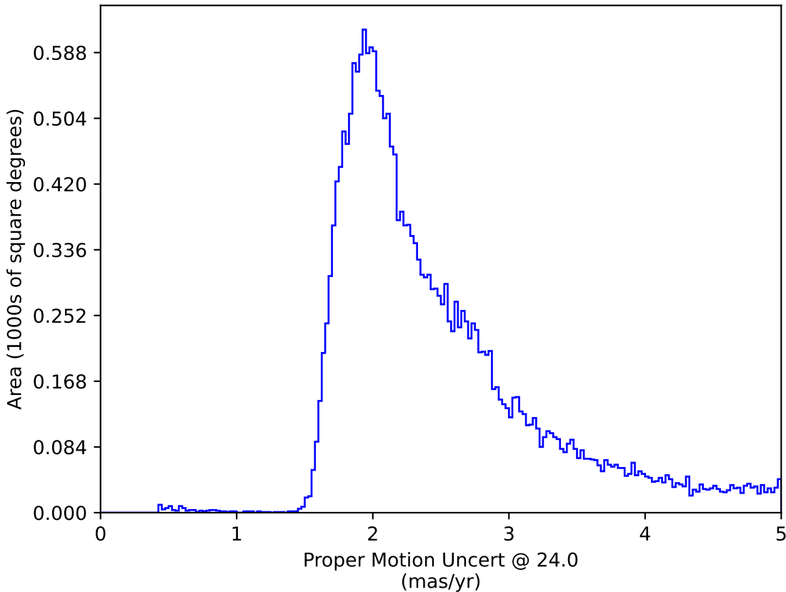
too_10_1v3.4_10yrs All sky: Proper Motion Uncert @ 24.0
