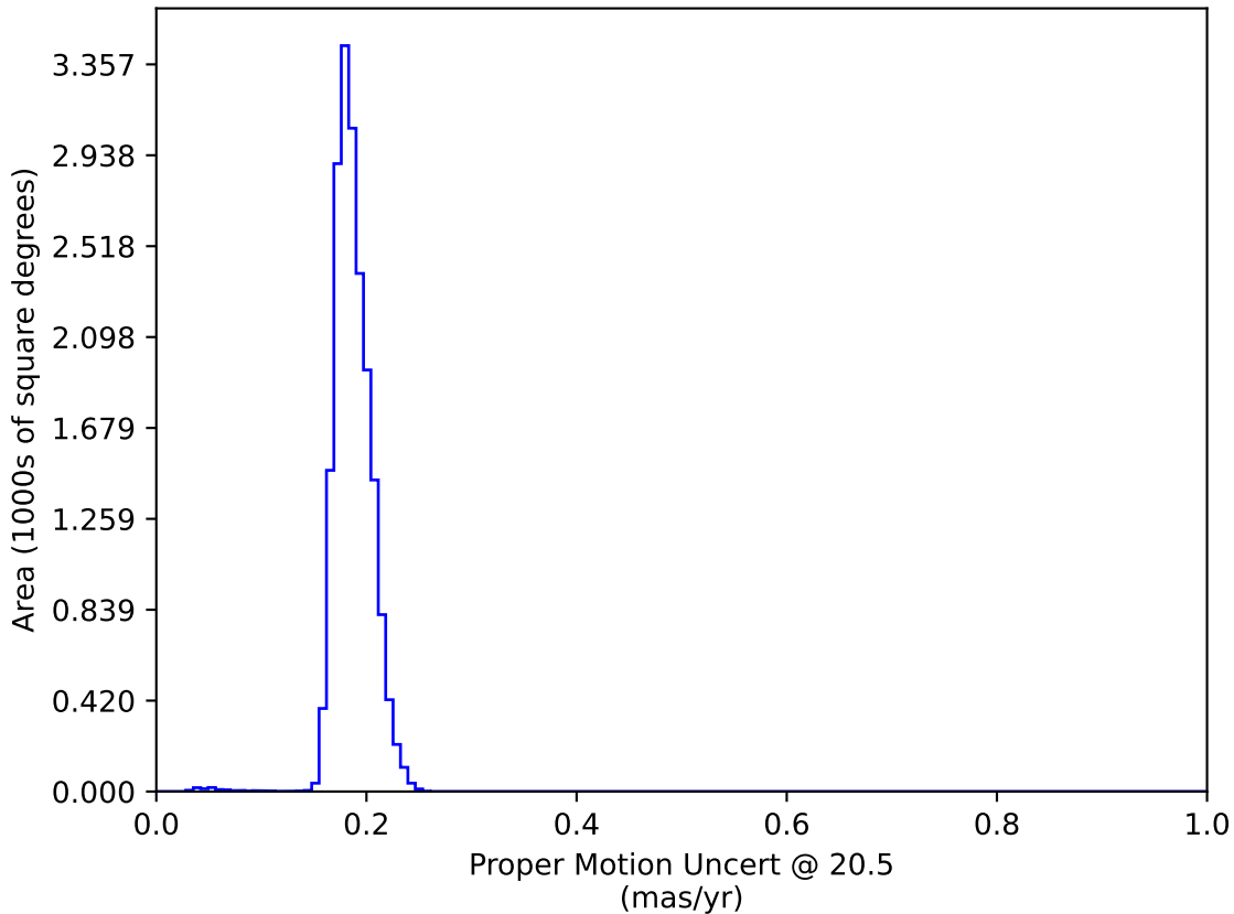
too_10_1v3.4_10yrs WFD: Proper Motion Uncert @ 20.5
