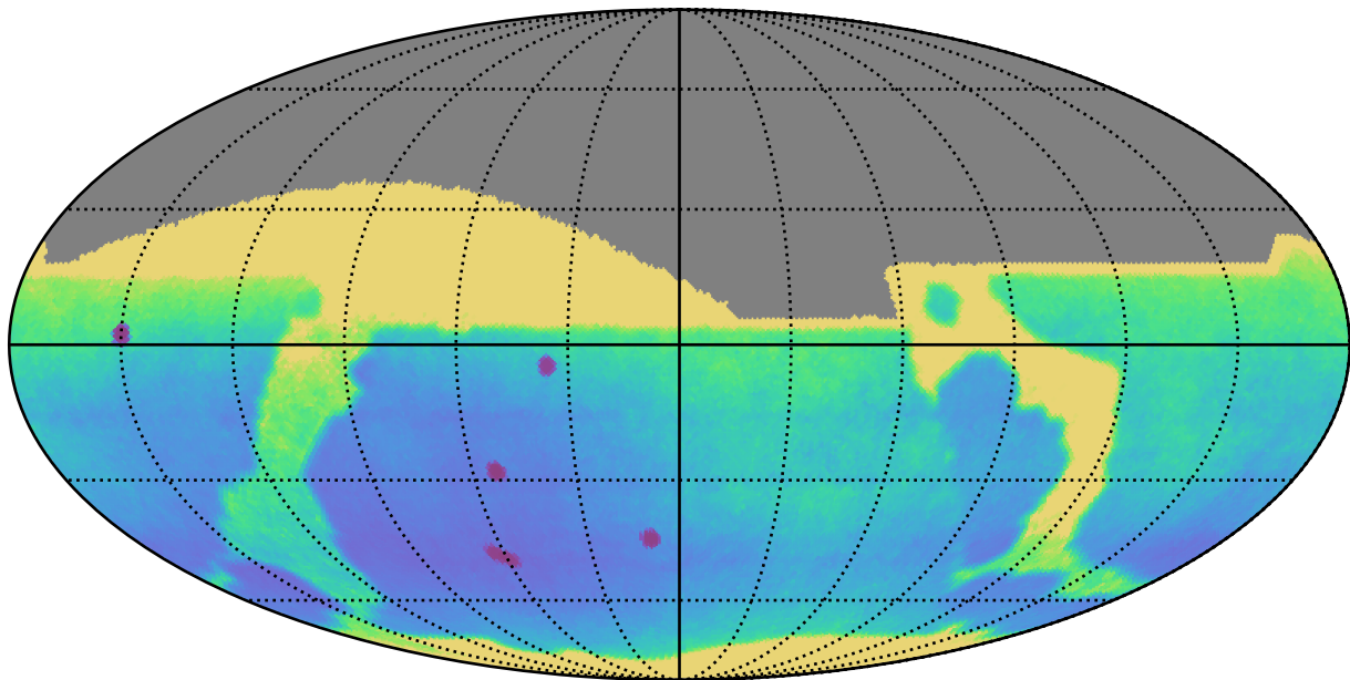
too_10_1v3.4_10yrs All sky: Parallax Uncert @ 24.0
