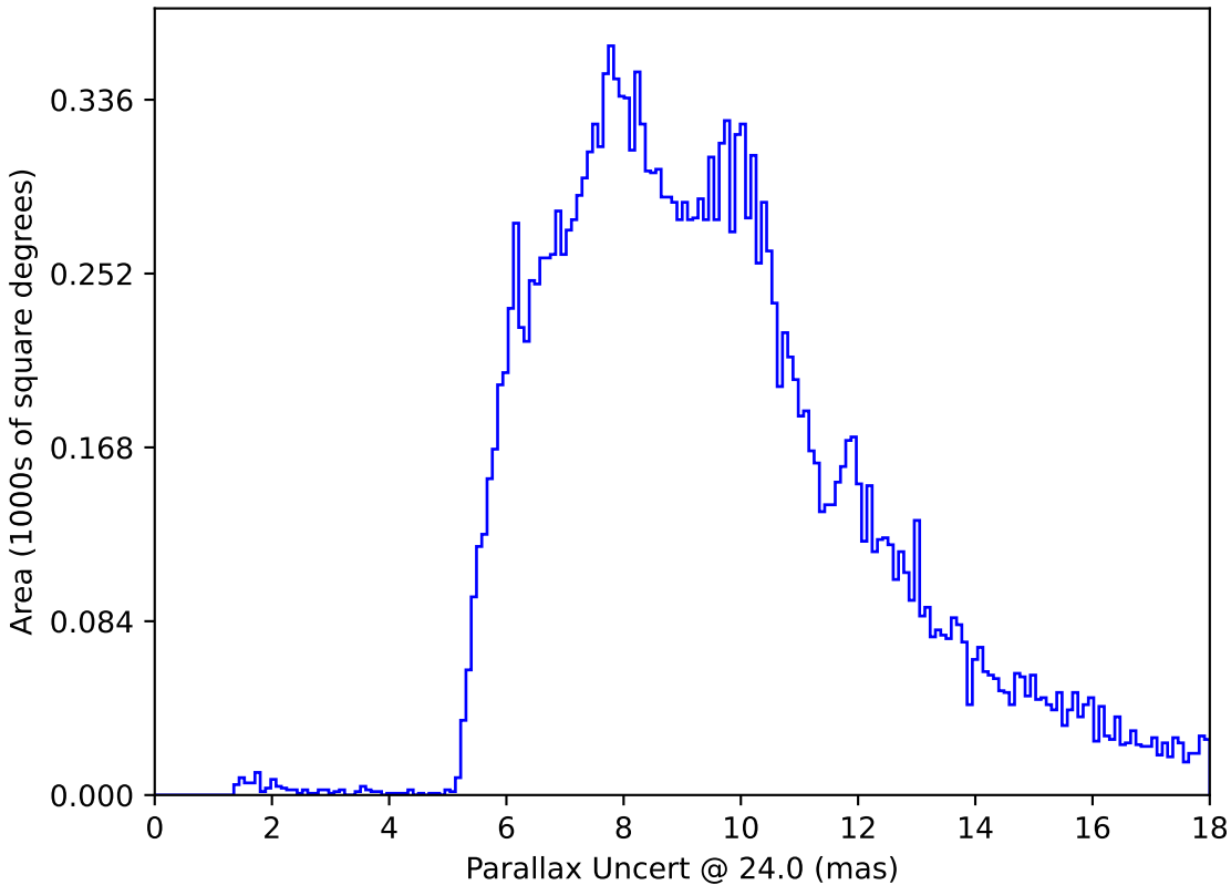
too_10_1v3.4_10yrs All sky: Parallax Uncert @ 24.0
