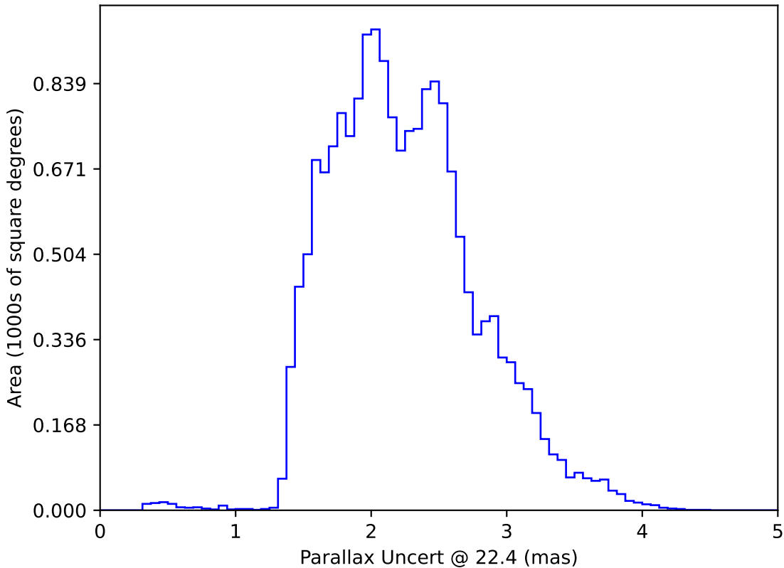
too_10_1v3.4_10yrs WFD: Parallax Uncert @ 22.4
