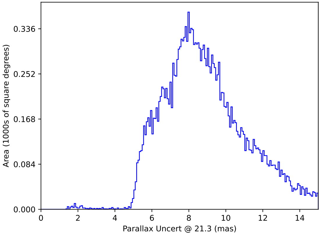
too_10_1v3.4_10yrs All sky y band only: Parallax Uncert @ 21.3
