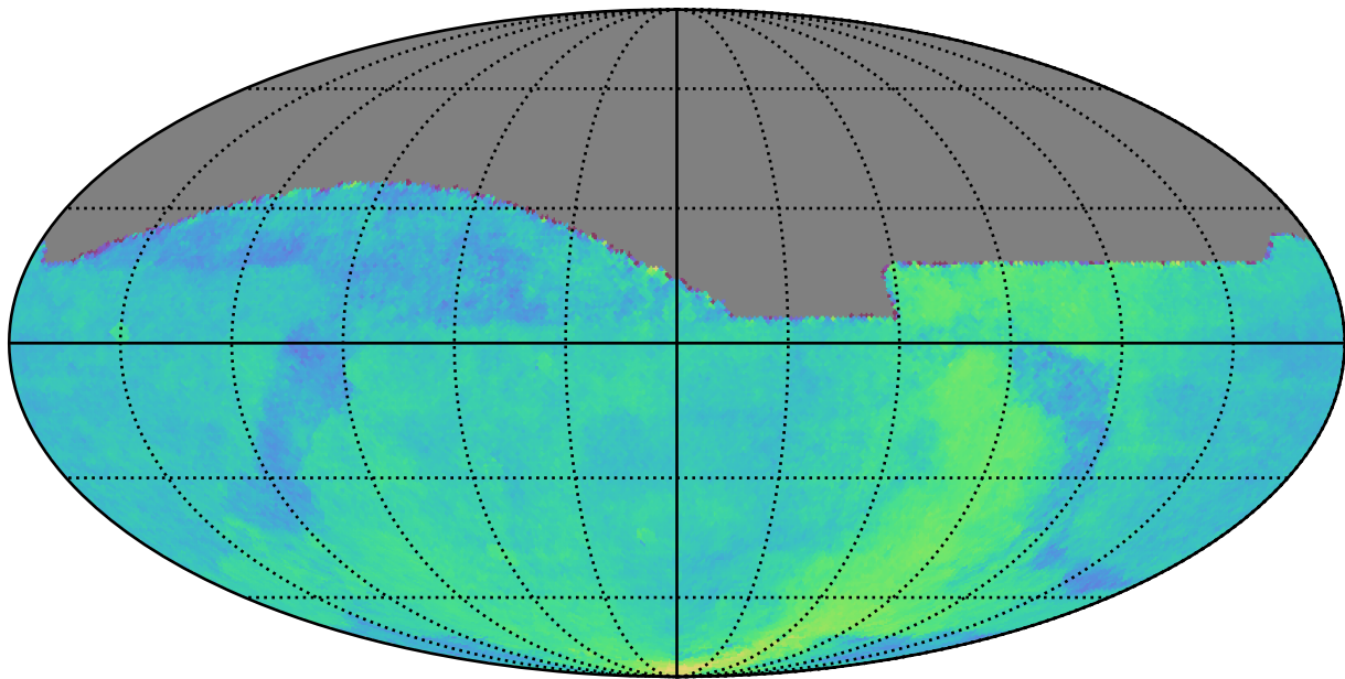
too_10_1v3.4_10yrs All sky: Parallax Coverage @ 24.0
