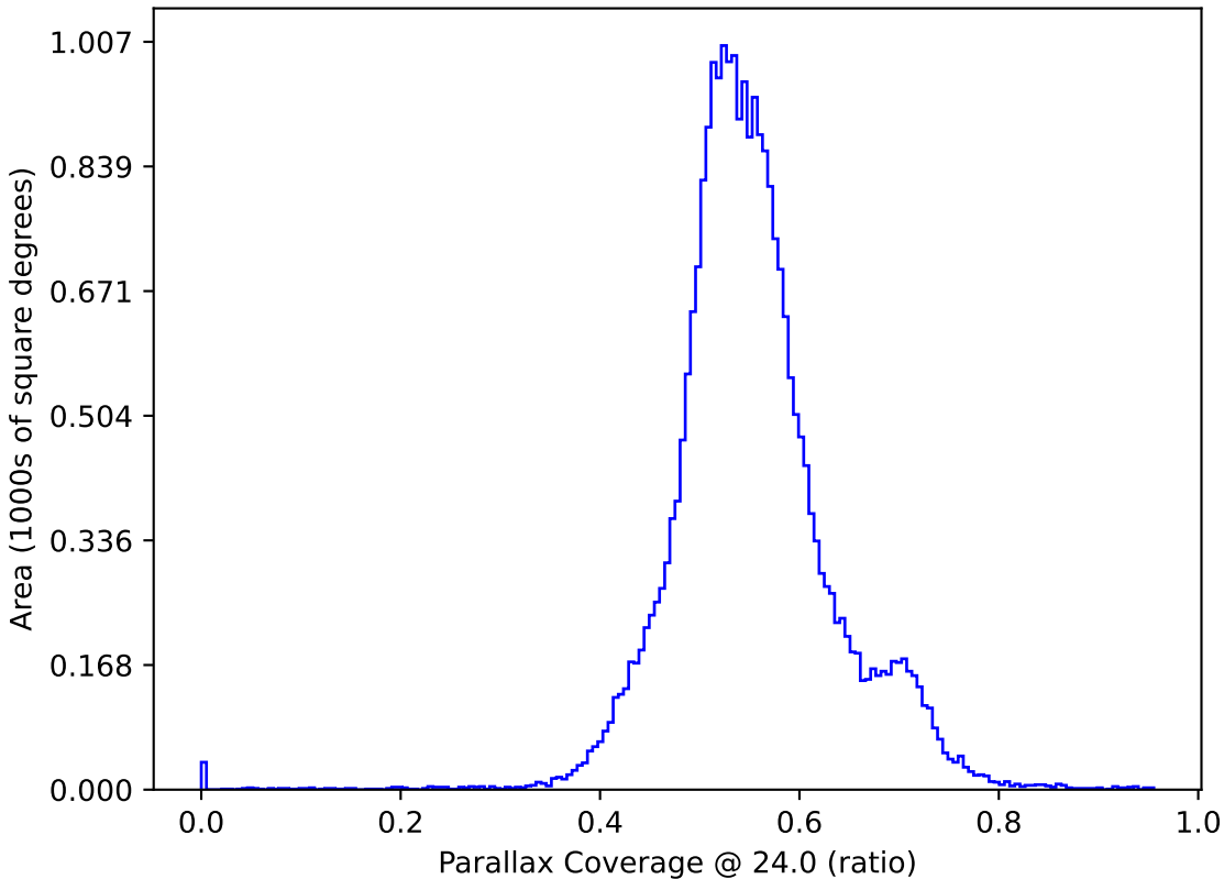
too_10_1v3.4_10yrs All sky: Parallax Coverage @ 24.0
