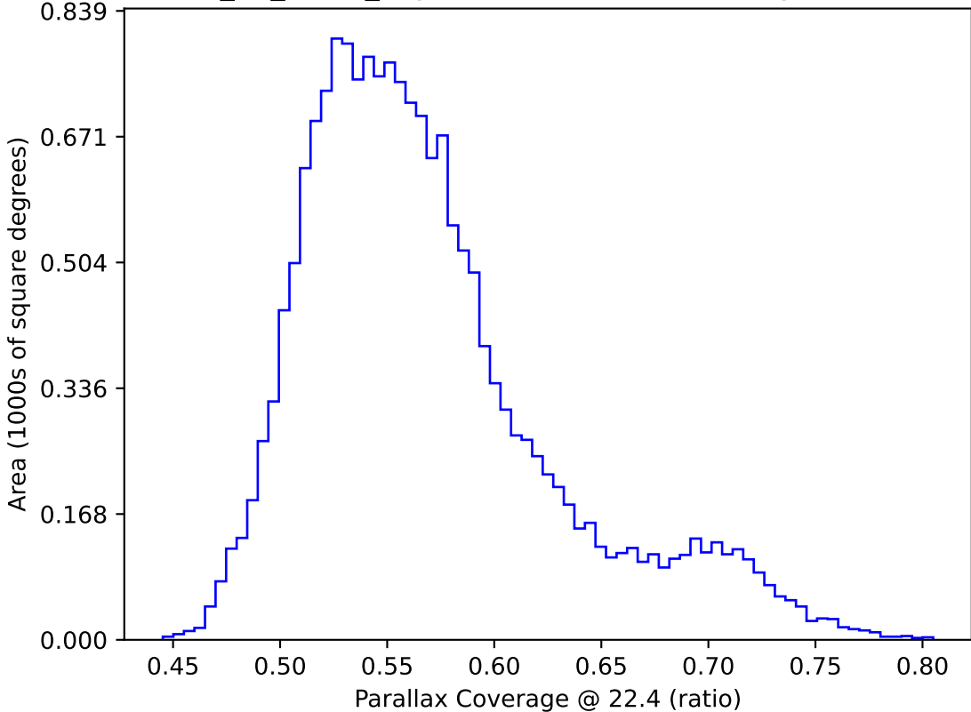
too_10_1v3.4_10yrs WFD: Parallax Coverage @ 22.4
