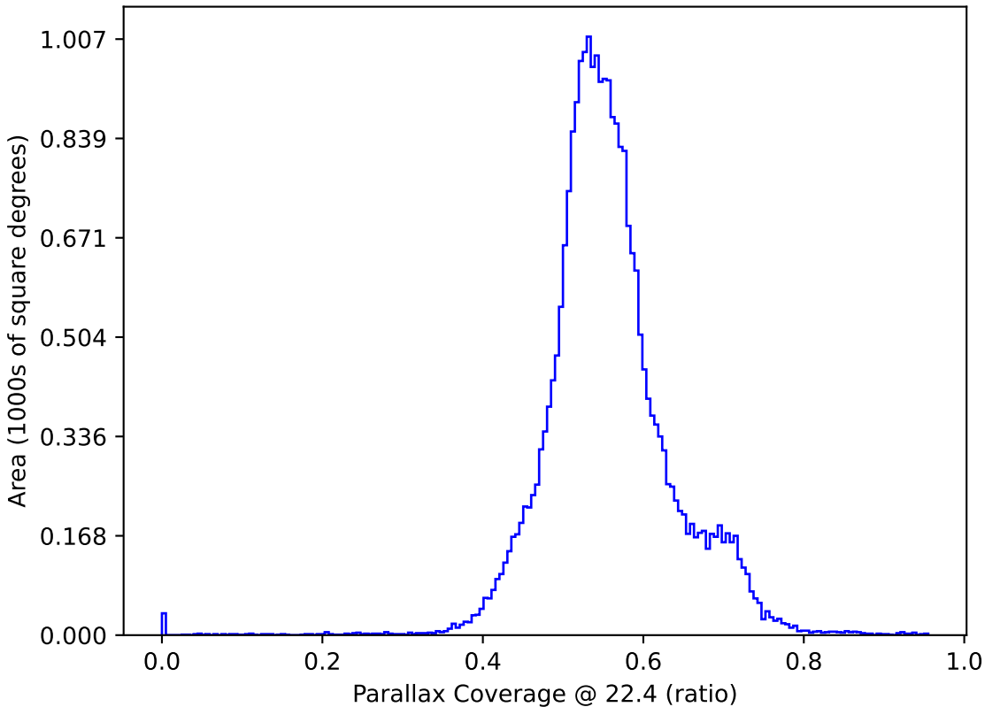
too_10_1v3.4_10yrs All sky: Parallax Coverage @ 22.4
