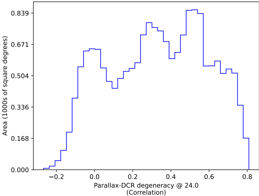
too_10_1v3.4_10yrs WFD: Parallax-DCR degeneracy @ 24.0
