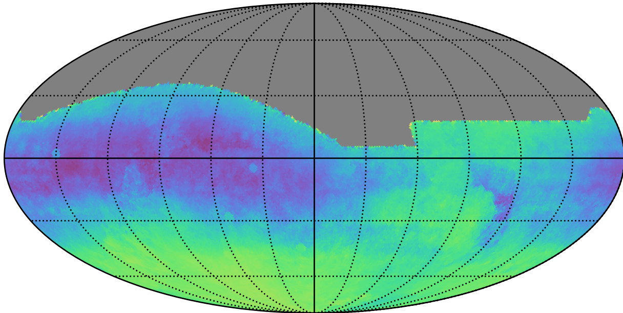
too_10_1v3.4_10yrs All sky: Parallax-DCR degeneracy @ 24.0
