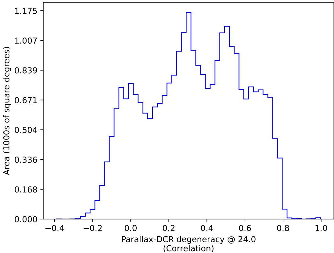
too_10_1v3.4_10yrs All sky: Parallax-DCR degeneracy @ 24.0
