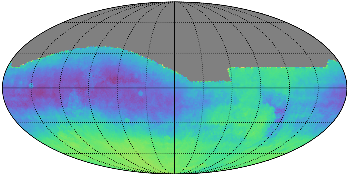
too_10_1v3.4_10yrs All sky: Parallax-DCR degeneracy @ 22.4
