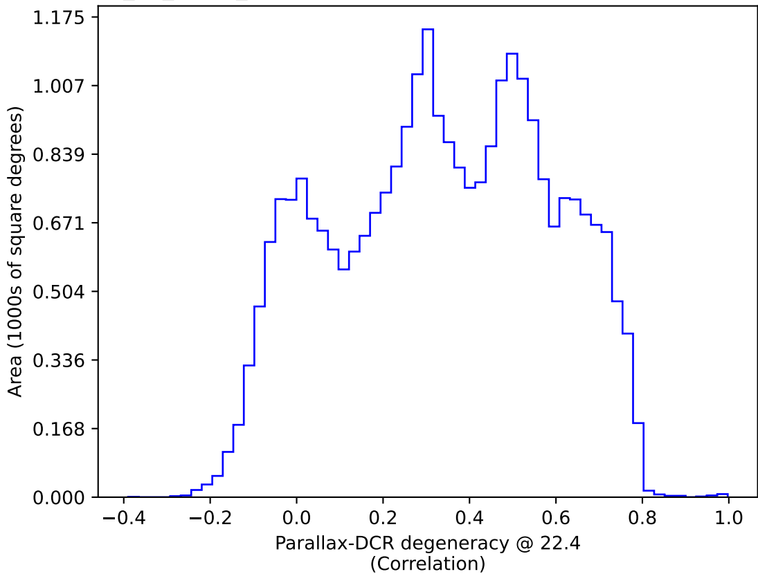
too_10_1v3.4_10yrs All sky: Parallax-DCR degeneracy @ 22.4
