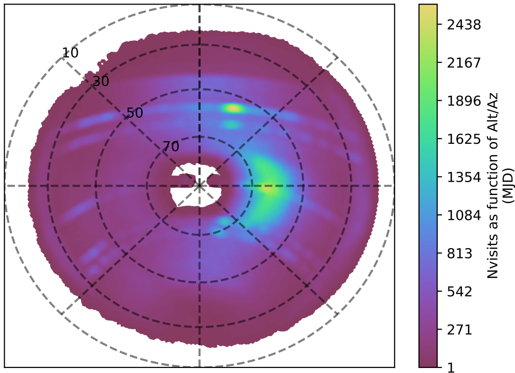
too_10_1v3.4_10yrs z band: Nvisits as function of Alt/Az
