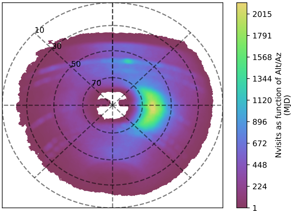
too_10_1v3.4_10yrs y band: Nvisits as function of Alt/Az
