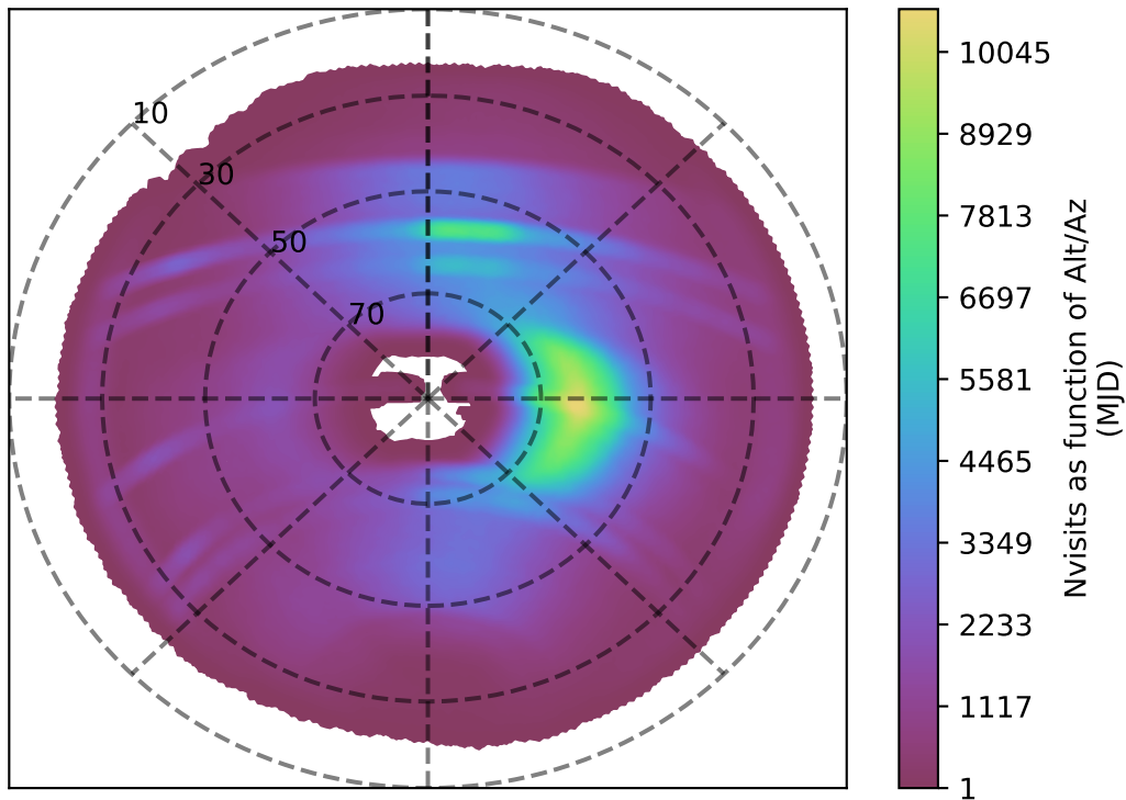
too_10_1v3.4_10yrs all bands: Nvisits as function of Alt/Az
